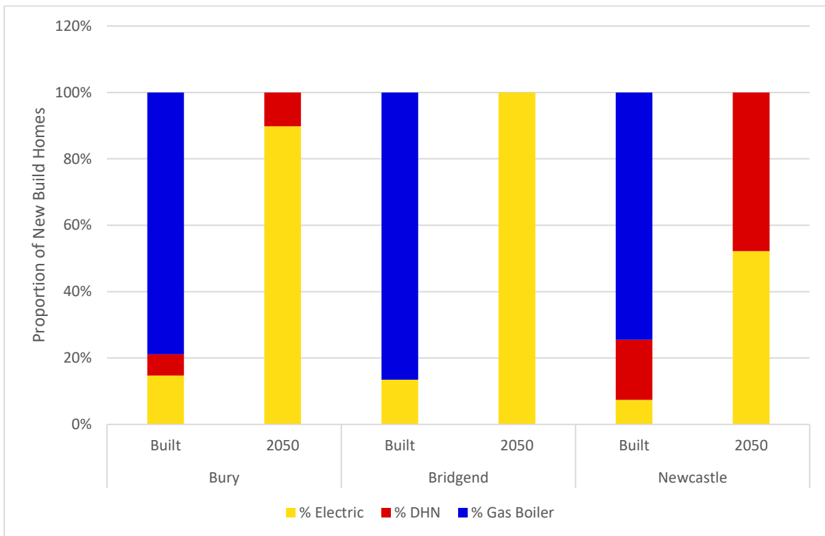
Figure 11: Heating systems fitted to new build homes when built and retrofitted to meet a 2050 carbon target.
