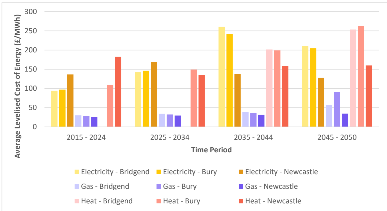
Figure 17: Example levelised costs of delivered energy for 3 different local areas
