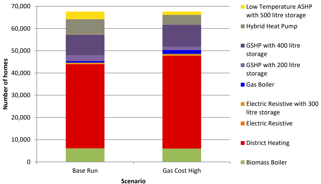
Figure 12: Comparison of domestic heating system solutions in Bridgend with different gas costs
