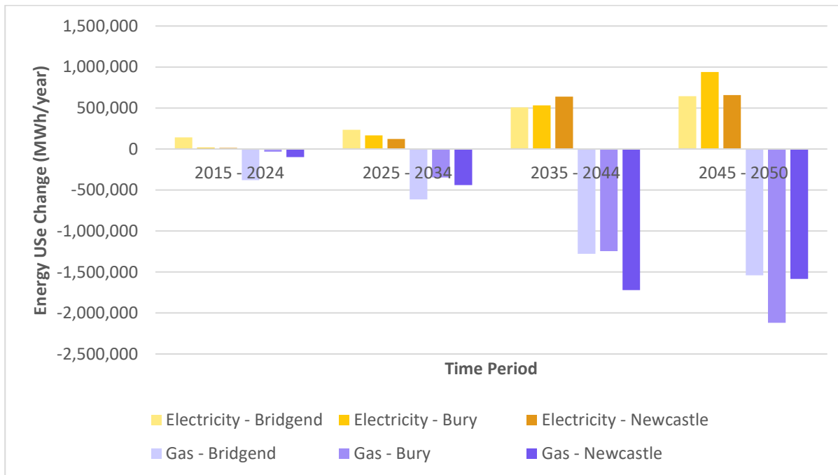
Figure 20: Example of annual energy savings resulting from decarbonisation for 3 different local areas
