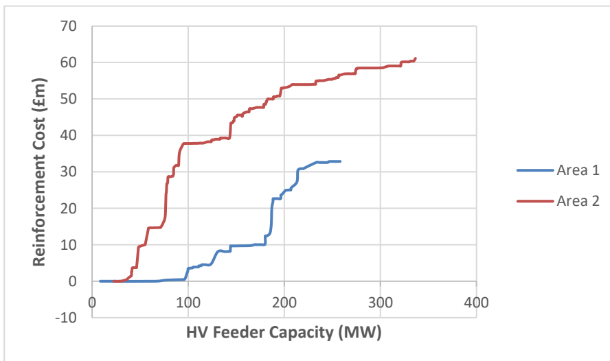
Figure 6: HV feeder network reinforcement cost curves for two areas in Bridgend
