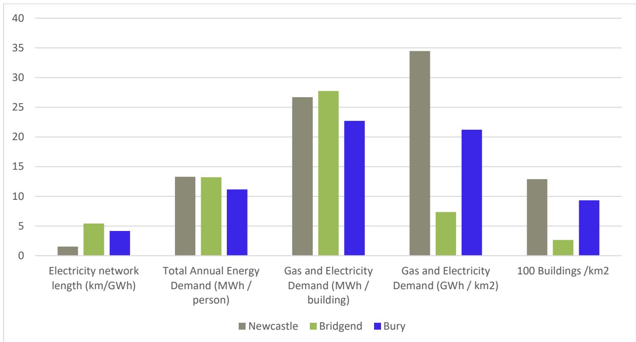
Figure 2: Normalised characteristics for three different areas
