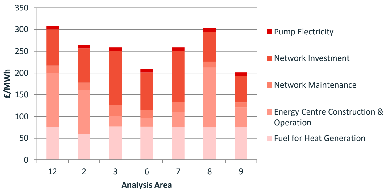
Figure 25: Delivered heat cost for heat networks in different areas of Bridgend
