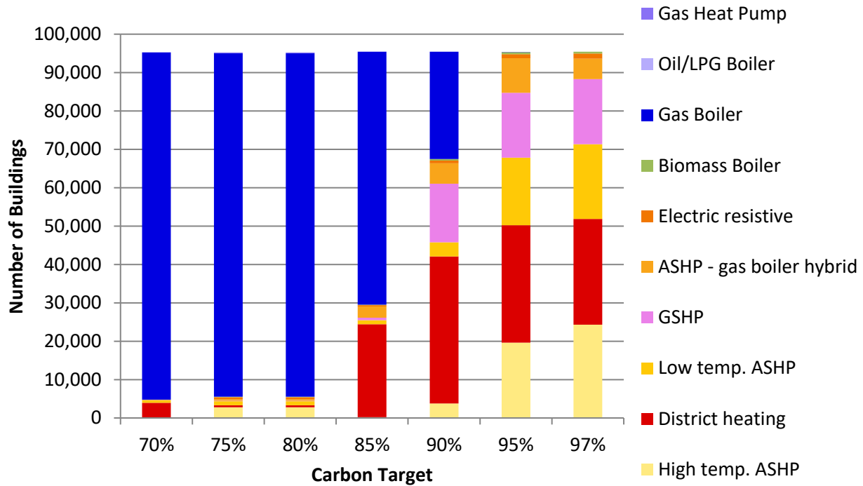
Figure 18: influence of local carbon target on heating system deployment in Bury
