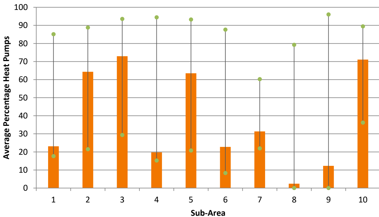
Figure 14: Ranges and average numbers of heat pumps selected for different scenarios in the Bridgend study
