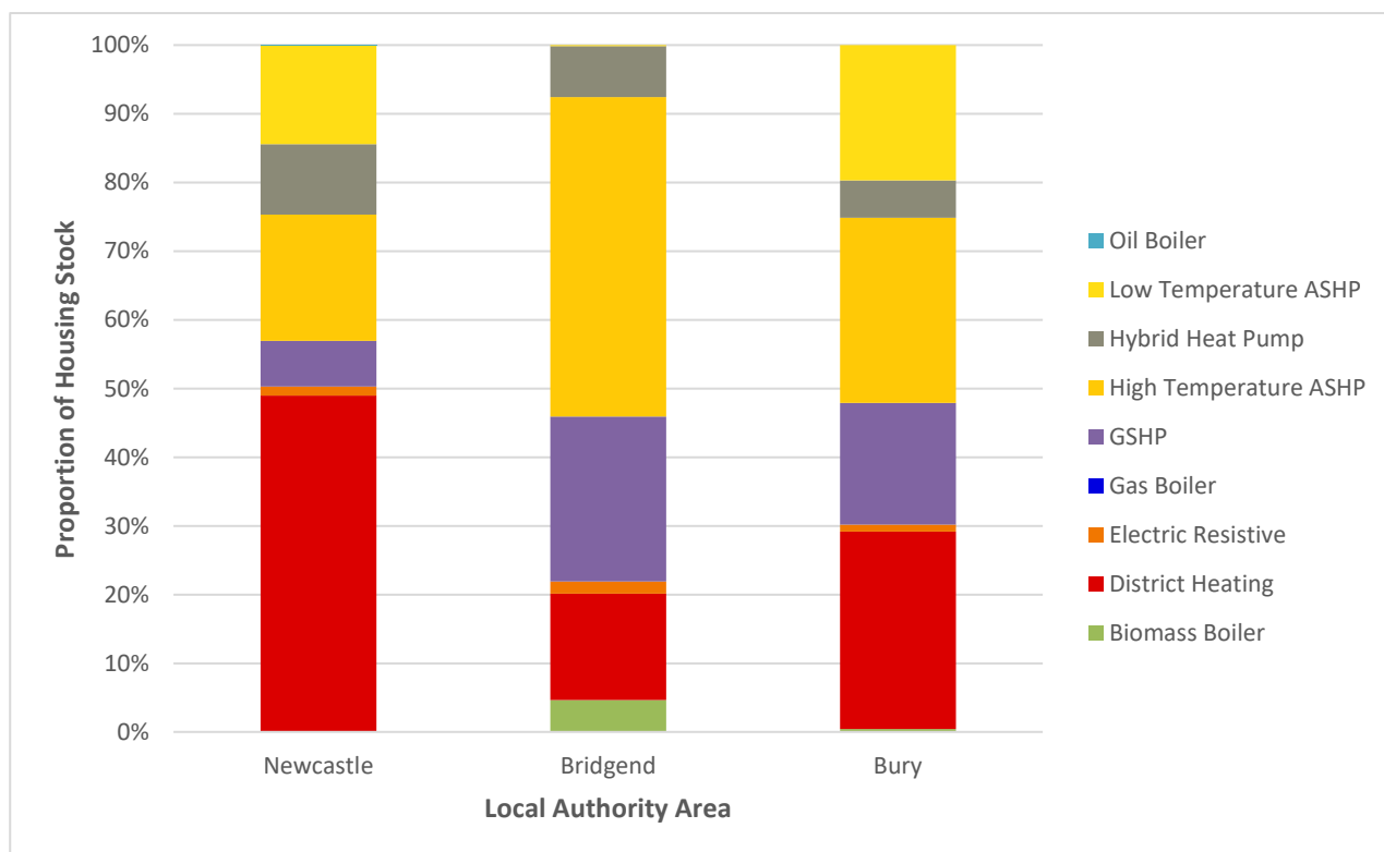
Figure 13: Proportion of different domestic heating solutions installed by 2050
