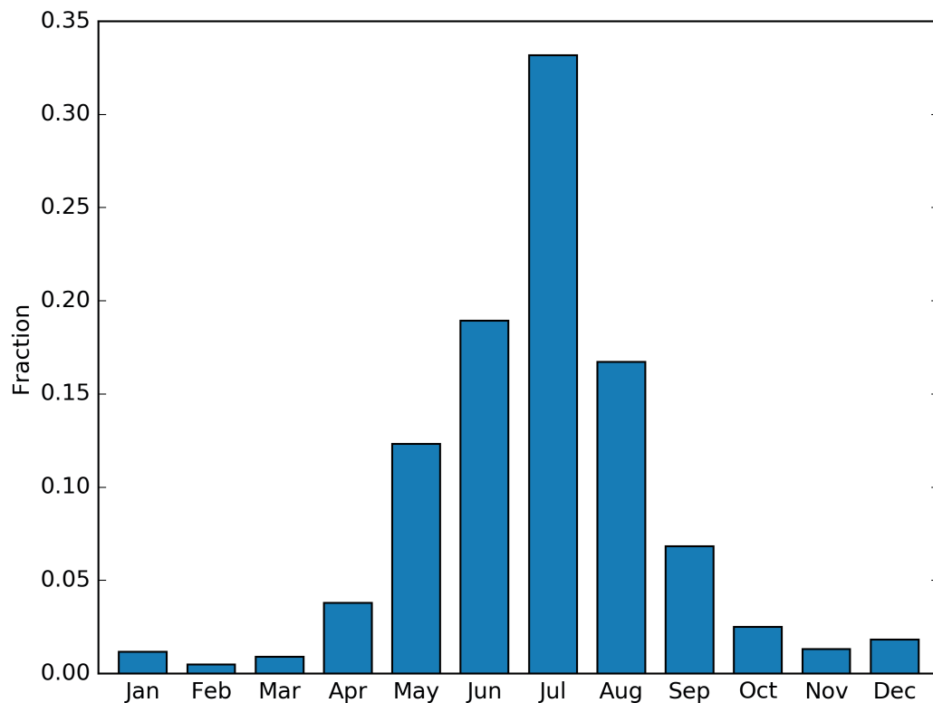
Figure 3. Fraction of lightning flashes per month recorded by ATDnet between 2008 and 2017.
