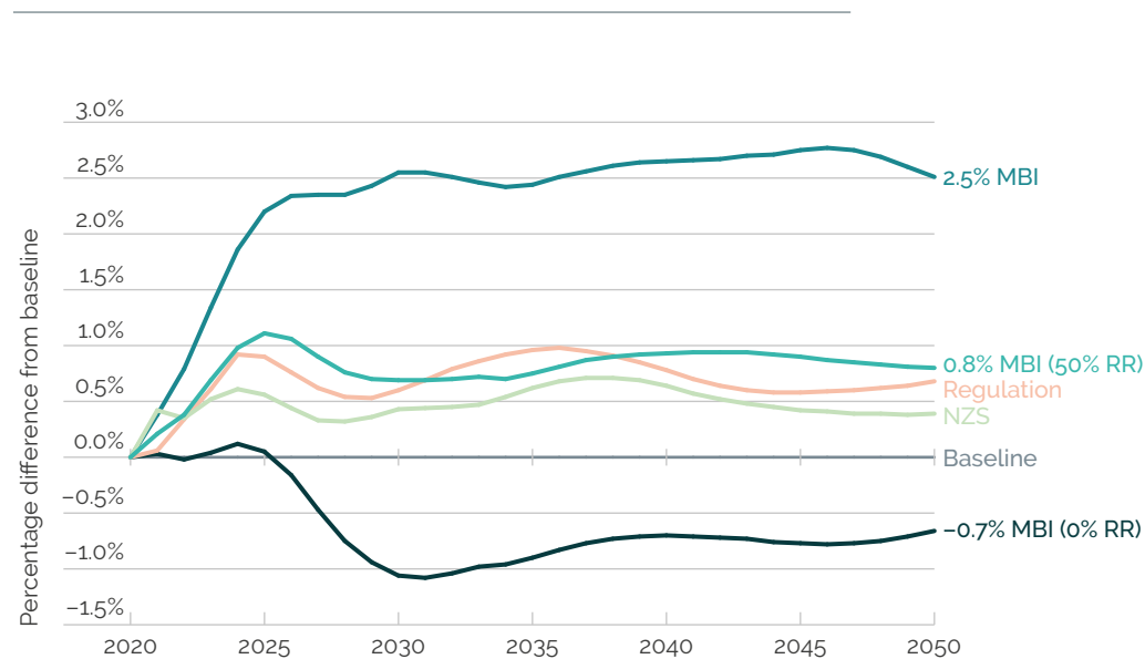
Figure 2.3: GDP by MBI revenue recycling sensitivity, relative differences from baseline, 2020-50.
