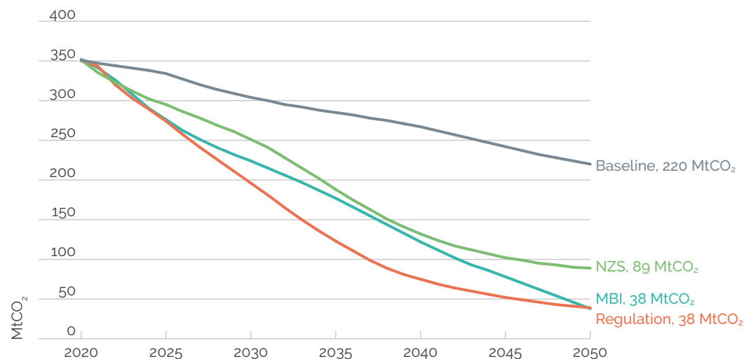
Figure 2.1: CO 2 emissions by scenario, MtCO 2 , 2020-50. Note: Includes CO 2 emissions from energy use and industrial processes only. The scenario outcomes put UK within range of net-zero once carbon removals from agriculture, forestry and land-use (AFOLU) and engineered removals are taken into account.
